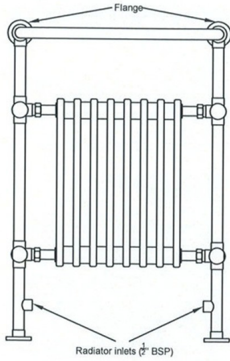
Floor mounted
